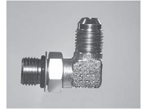
56725 9/16" O-Ring to JIC 90° Elbow
